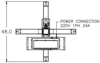
Front view SINGLE THERMORAY
